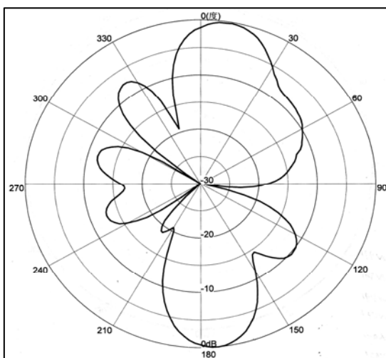
E-plane pattern
